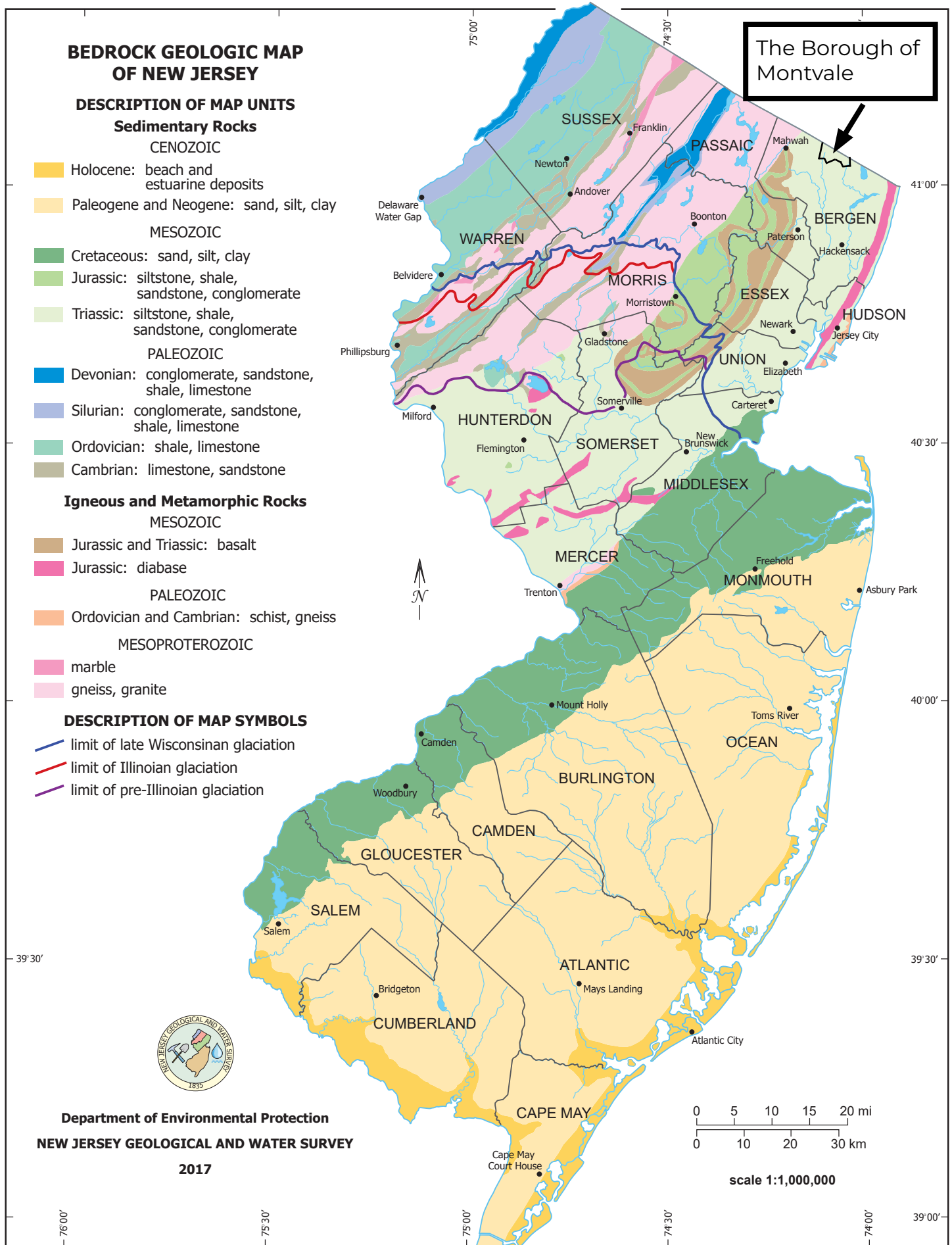
Figure 3. Bedrock Geology in New Jersey, NJDEP. https://www.nj.gov/dep/hjgs/NJMaps
