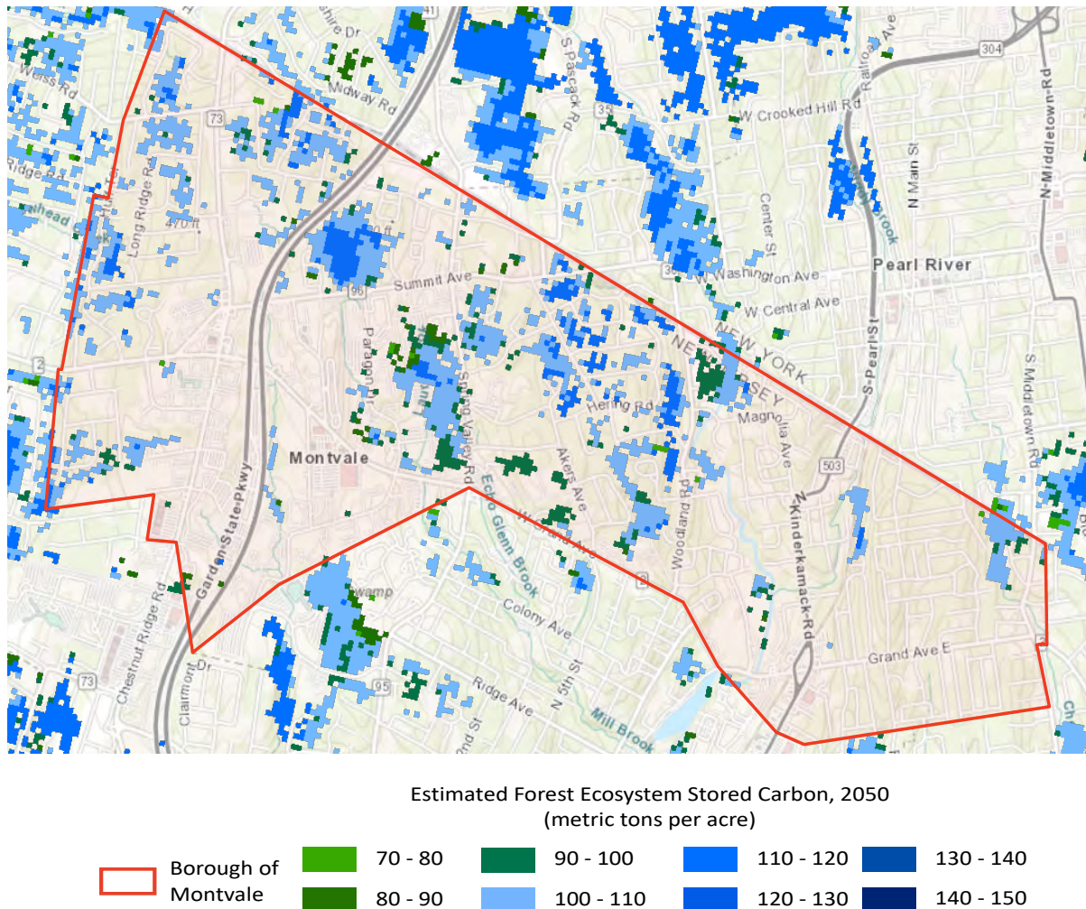
Figure 5. Estimated Forest Ecosystem Stored Carbon, Montvale 2050. Resilient Land Mapping Tool- The Nature Conservancy.
